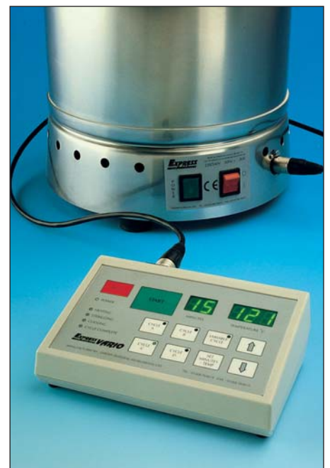
'Vario' controller in use
